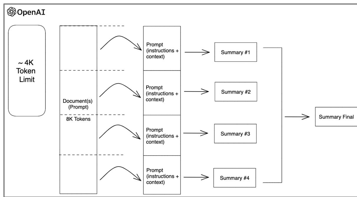
Map-Reduce
